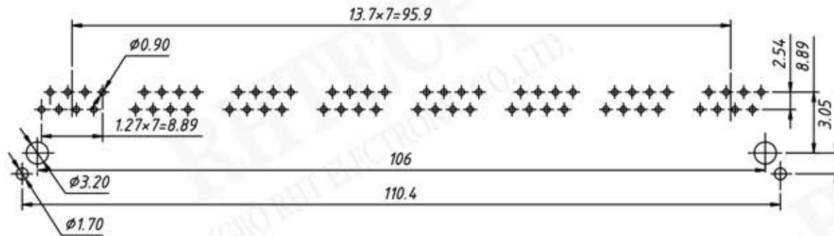
PCB Layout
